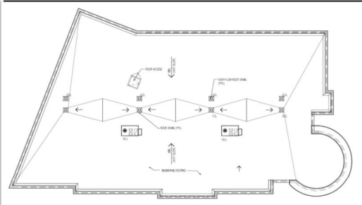
3 ROOF PLAN SCALE: 1/8" = 1'-0"
